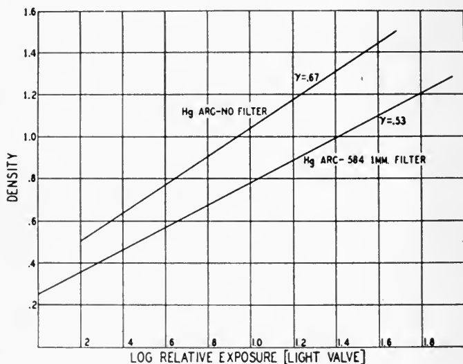
FIG. 5. Effect of ultraviolet filter on sound negative gamma.
